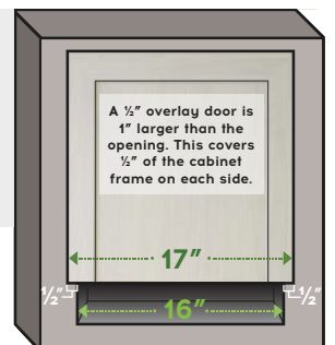
1/2" OVERLAY DOOR EXAMPLE
